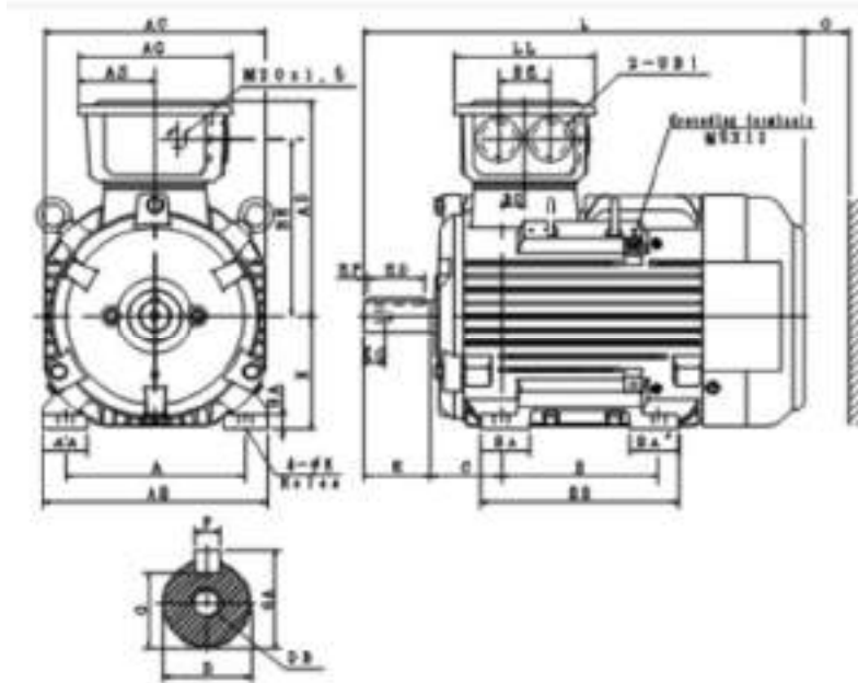
Figure 7-4: Outline drawing of cast iron design, feet version, mounting B3; frame size 80 – 112
