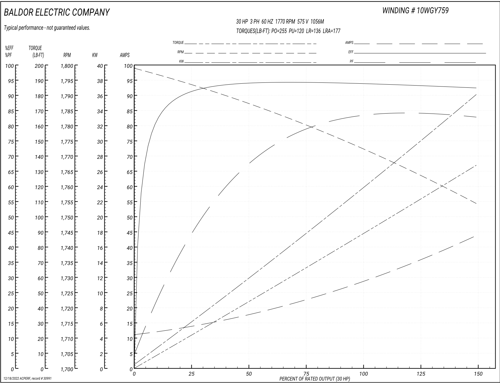
Performance Graph at 575V, 60Hz, 30.0HP Typical performance - Not guaranteed values
